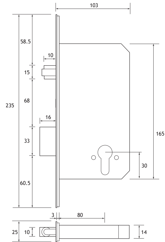
PR6131RBD Roller Bolt Dead lock
