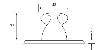
PR4-729A Anti-ligature Pull Handle
