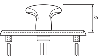
PR4-728TP Anti-ligature Thumb Turn/Pull
