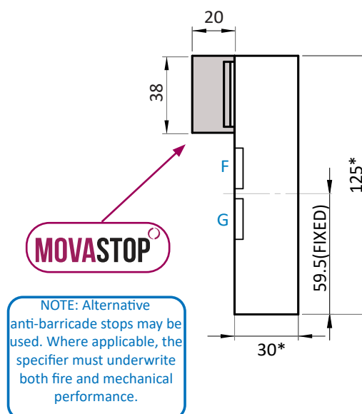
Closing Jamb
