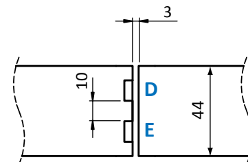
Meeting Stile
